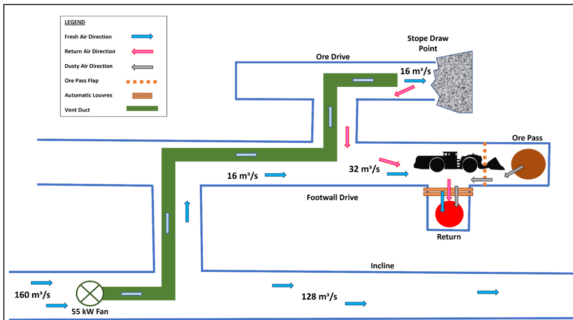
Figure 16-39 Example of a Production Level Ventilation Plan
