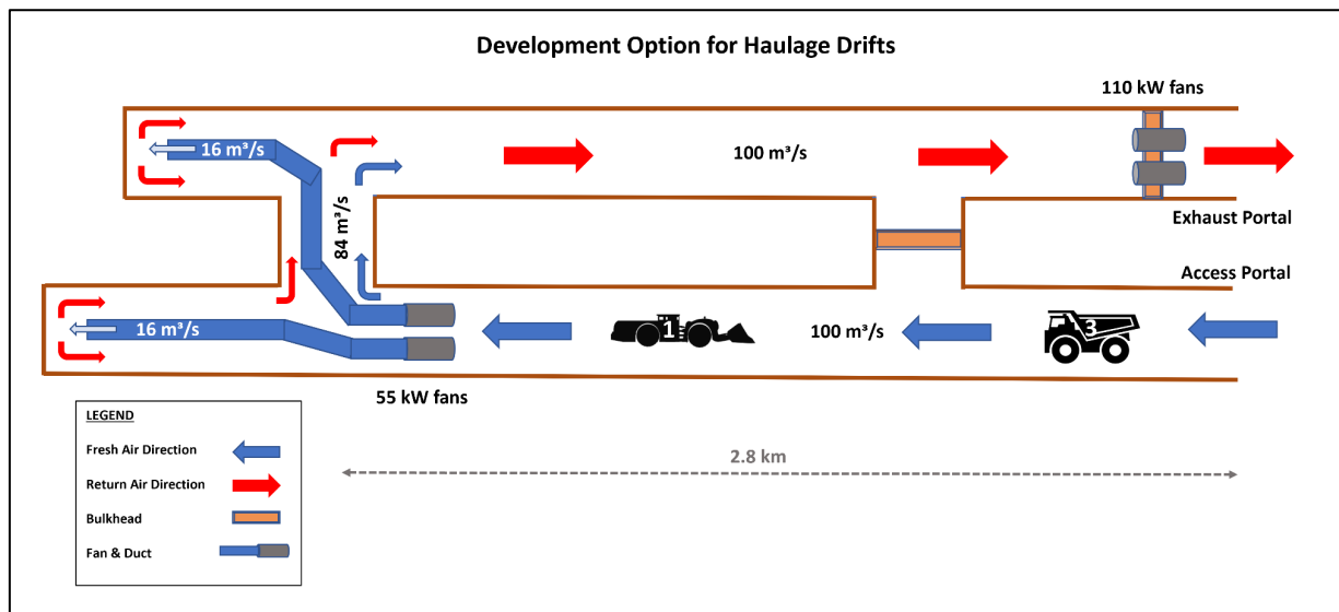
Figure 16-46 Initial Development Option for Haulage Drifts
