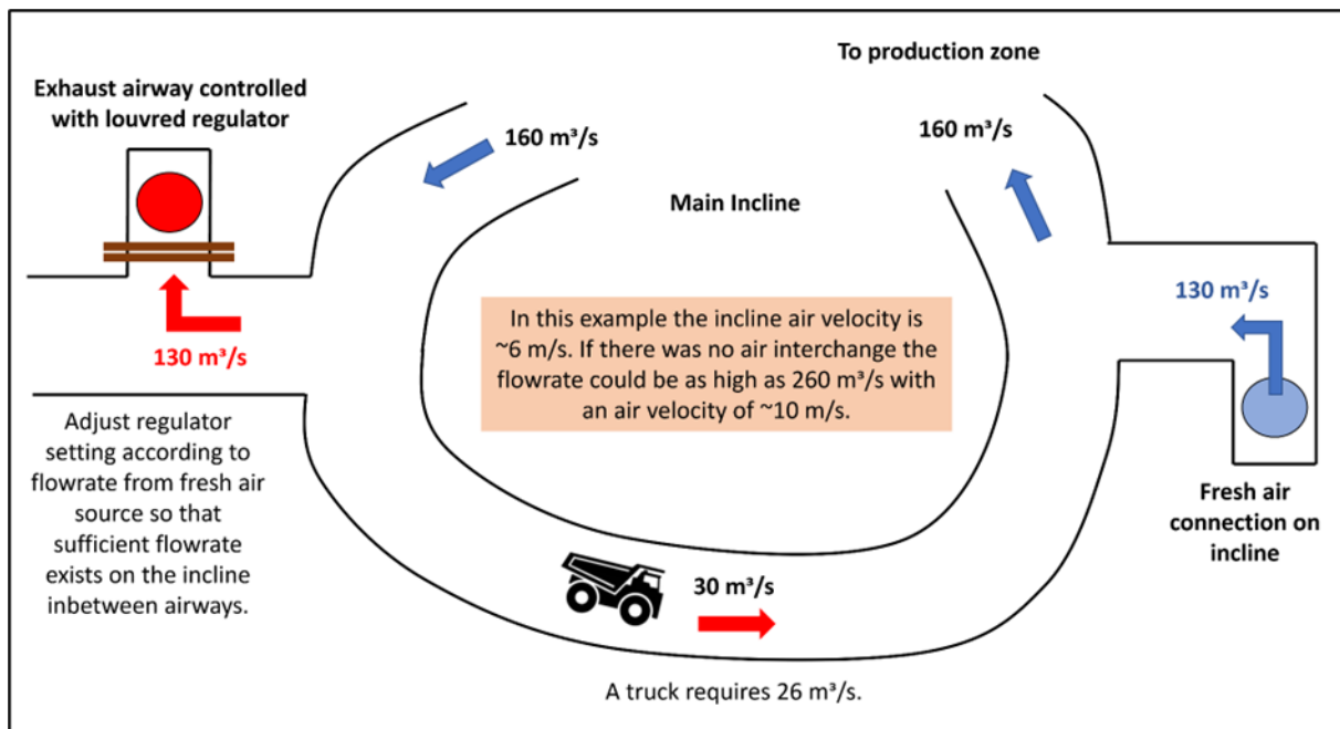
Figure 16-38 How an Air Interchange Works
