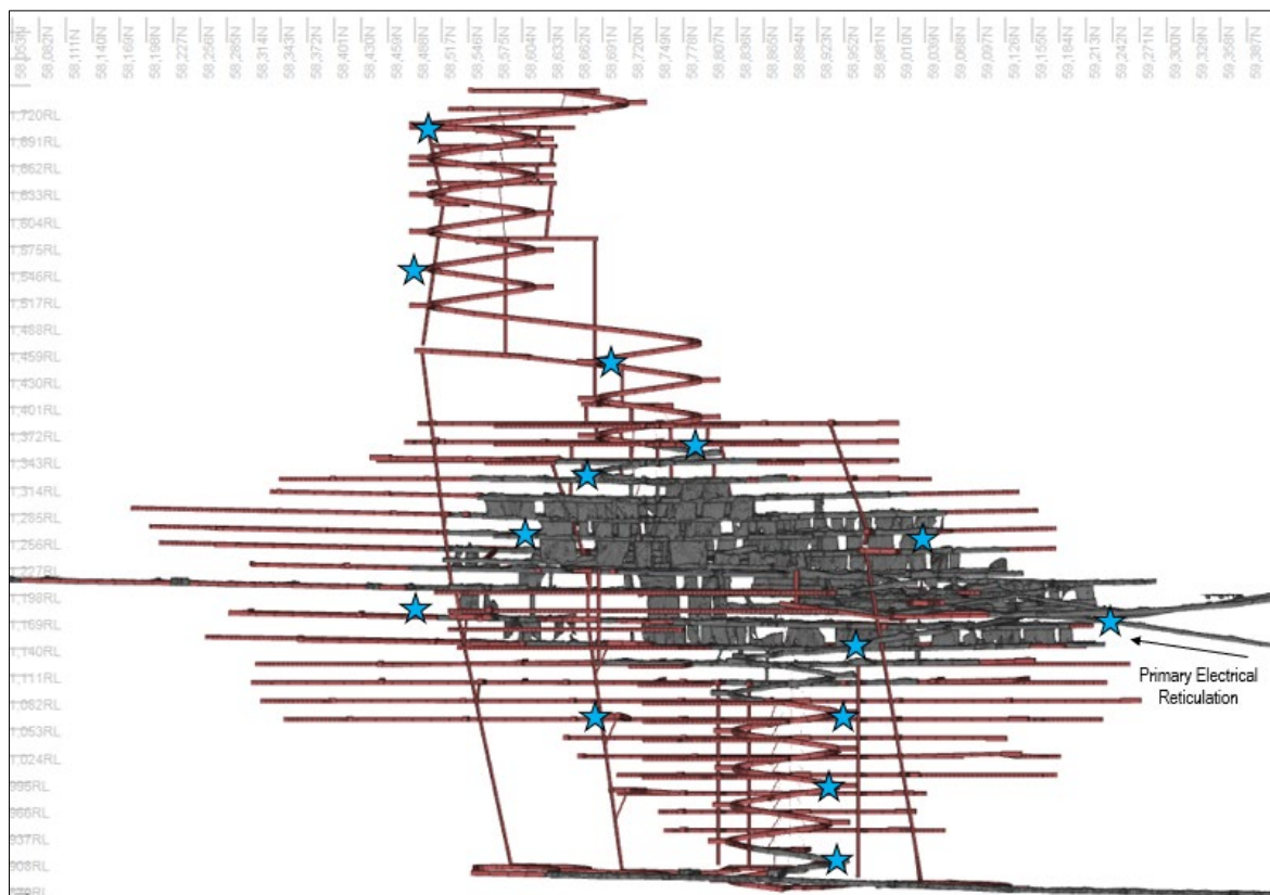
Figure 16-48 Estimated Underground Power Substation Network (Star Locations Depict Potential Placement of 2MW Substations)
