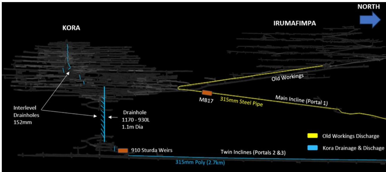
Figure 16-49 Overview Dewatering System
