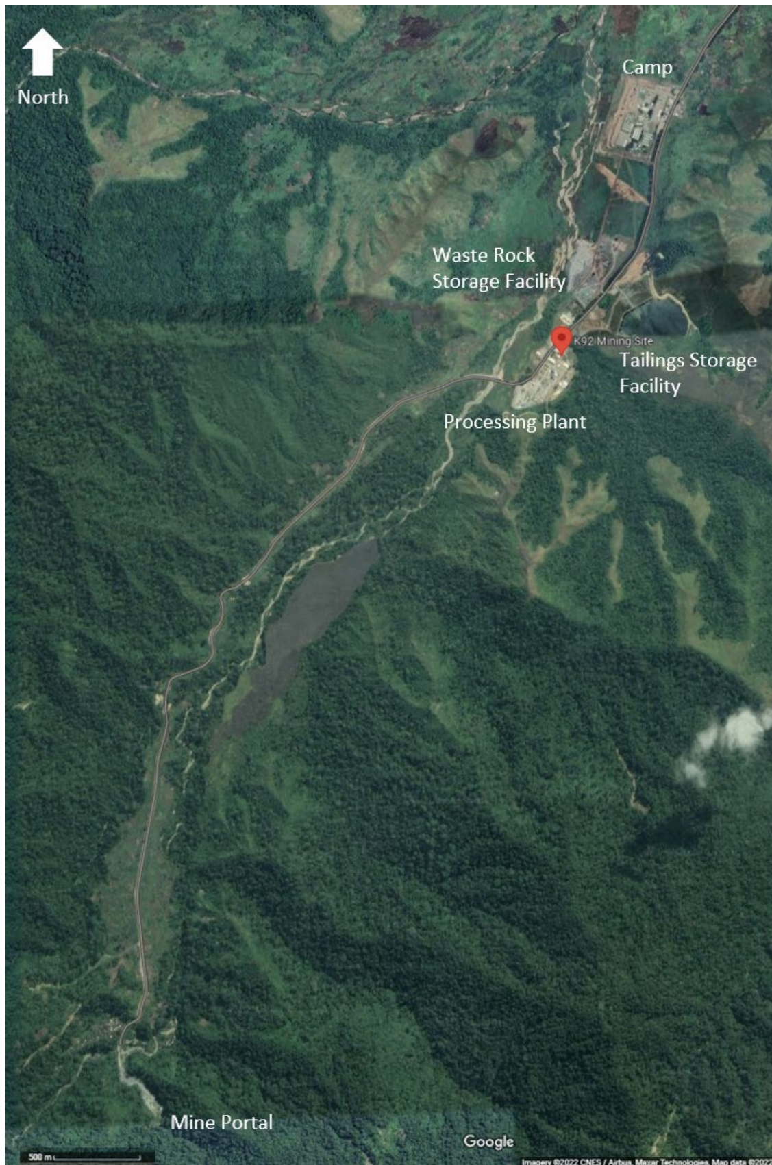
Figure 16-51 Overall Site Layout (~6 km From Mine Portal to Processing Plant)
