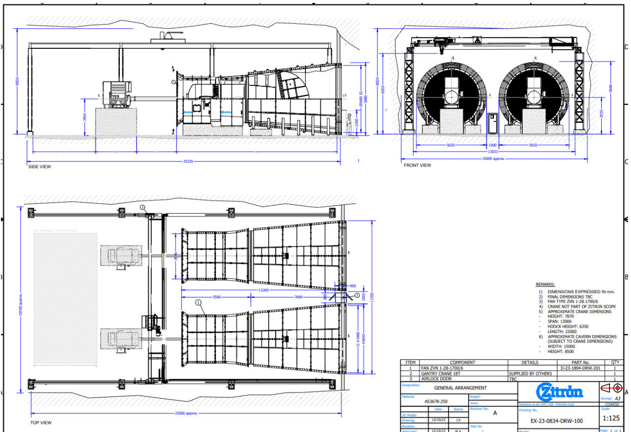
Figure 16-42 Overview of Underground Fan Station care of Zitron
