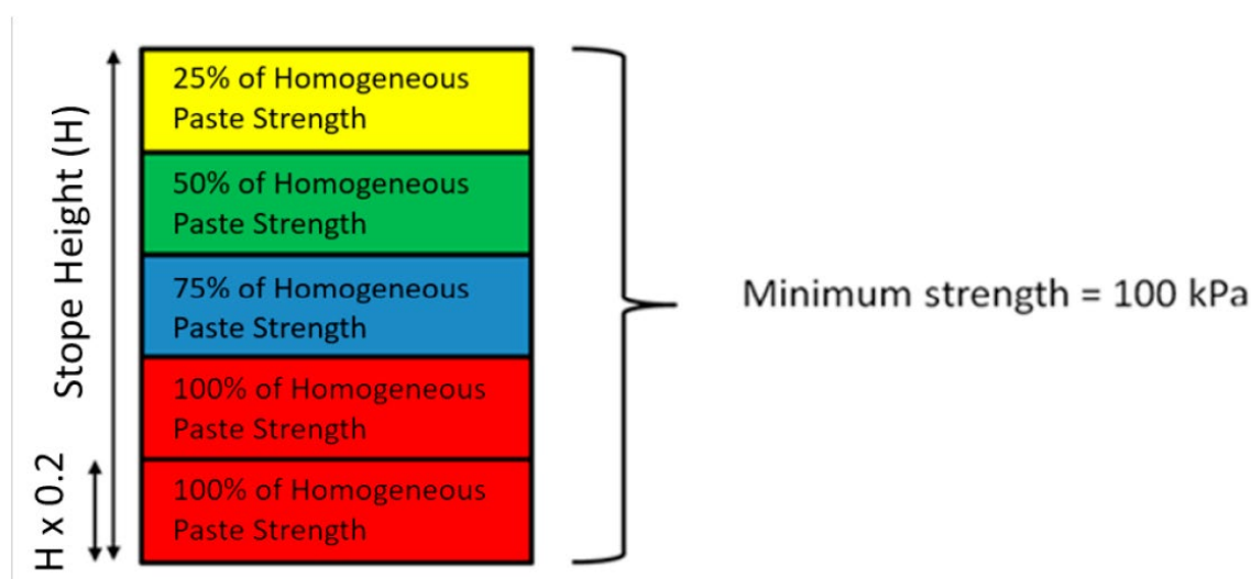
Figure 13-59 Fill Strength Reduction Criterion Simulated
