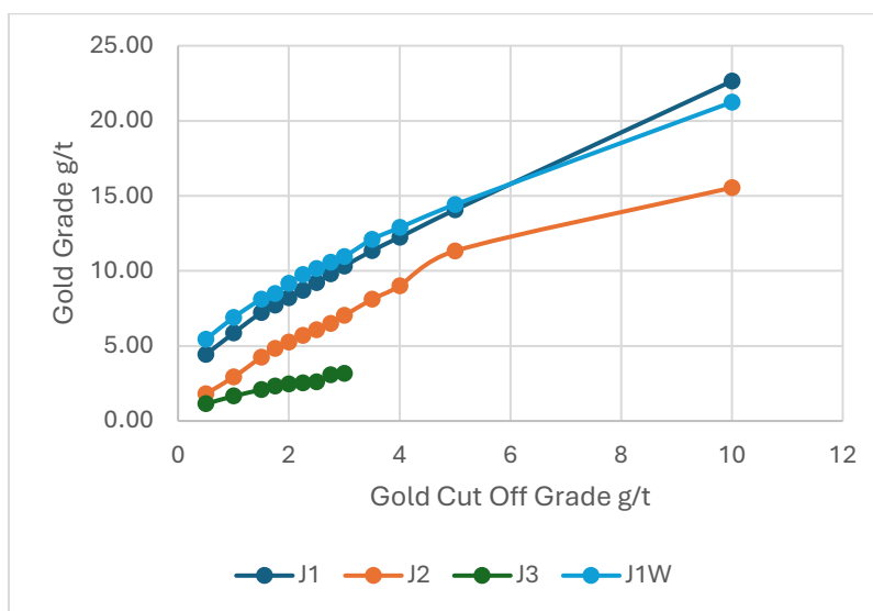
Figure 14-60 Gold Grade Curves for the Combined Judd Lodes (H&SC)
