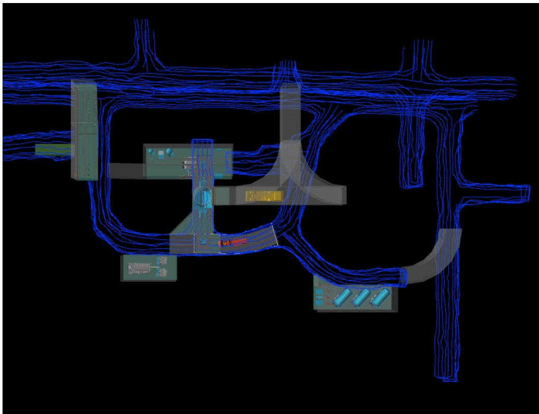
Figure 18-5 Paste Plant Infrastructure Top View (with access drifts shown)
