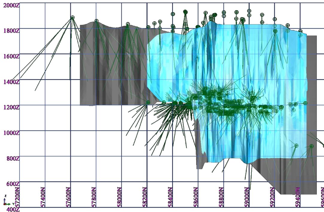
Figure 14-5 Long Section Comparison of the 2021 and 2023 K1 Mineral Lodes - looking west (H&SC)
