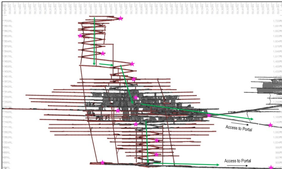
Figure 16-47 Proposed Underground Refuge Chambers (Purple) and Escapeway Route (Green arrows)
