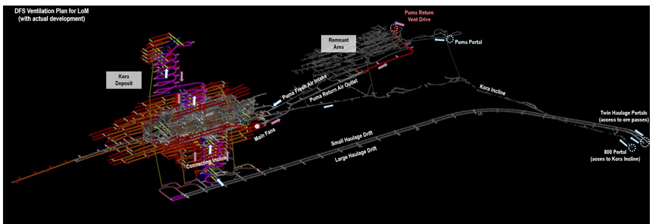
Figure 16-37: DFS LOM Ventilation Plan Profile Facing Northwest
