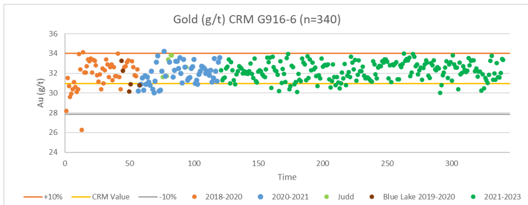
Figure 11-14 High Grade Standard (G916-6)
