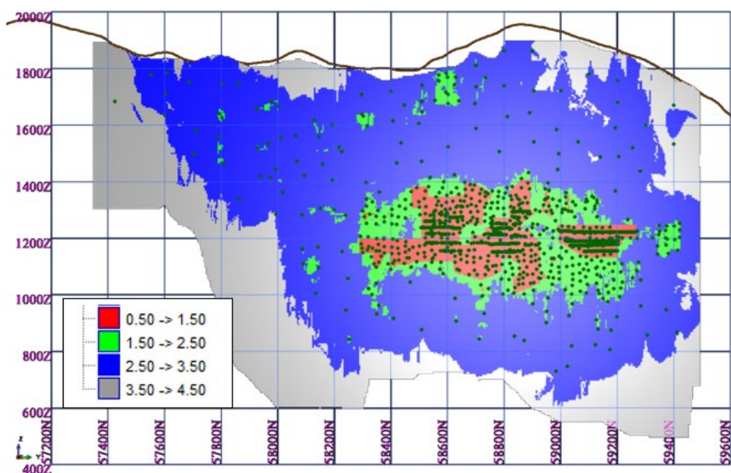
Figure 14-80 Resource Classification for the K1 Lode (H&SC)
