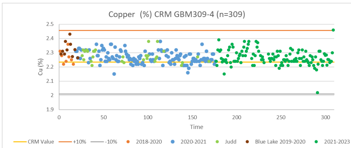
Figure 11-18 High Grade Copper Standard GBM309-4
